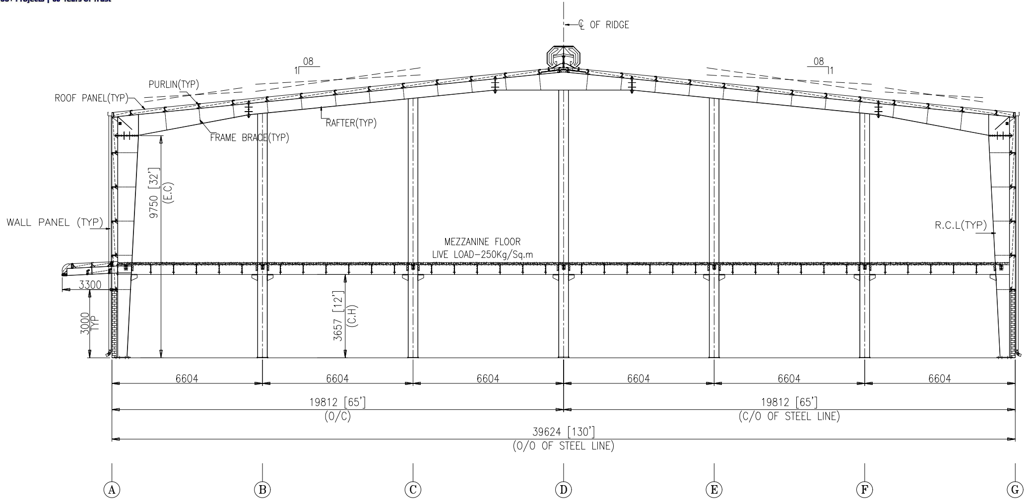
CROSS SECTION AT FRAME LINE-02
