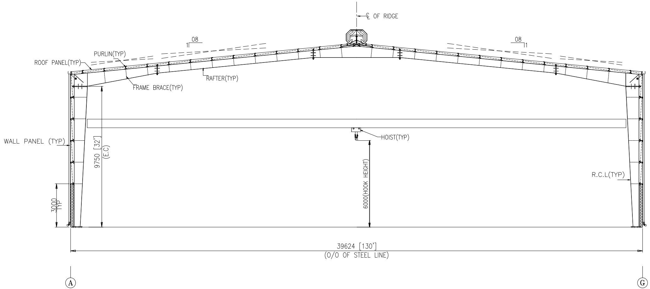
CROSS SECTION AT FRAME LINE-03
