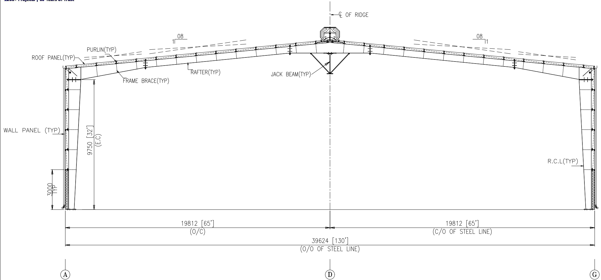
CROSS SECTION AT FRAME LINE-11
