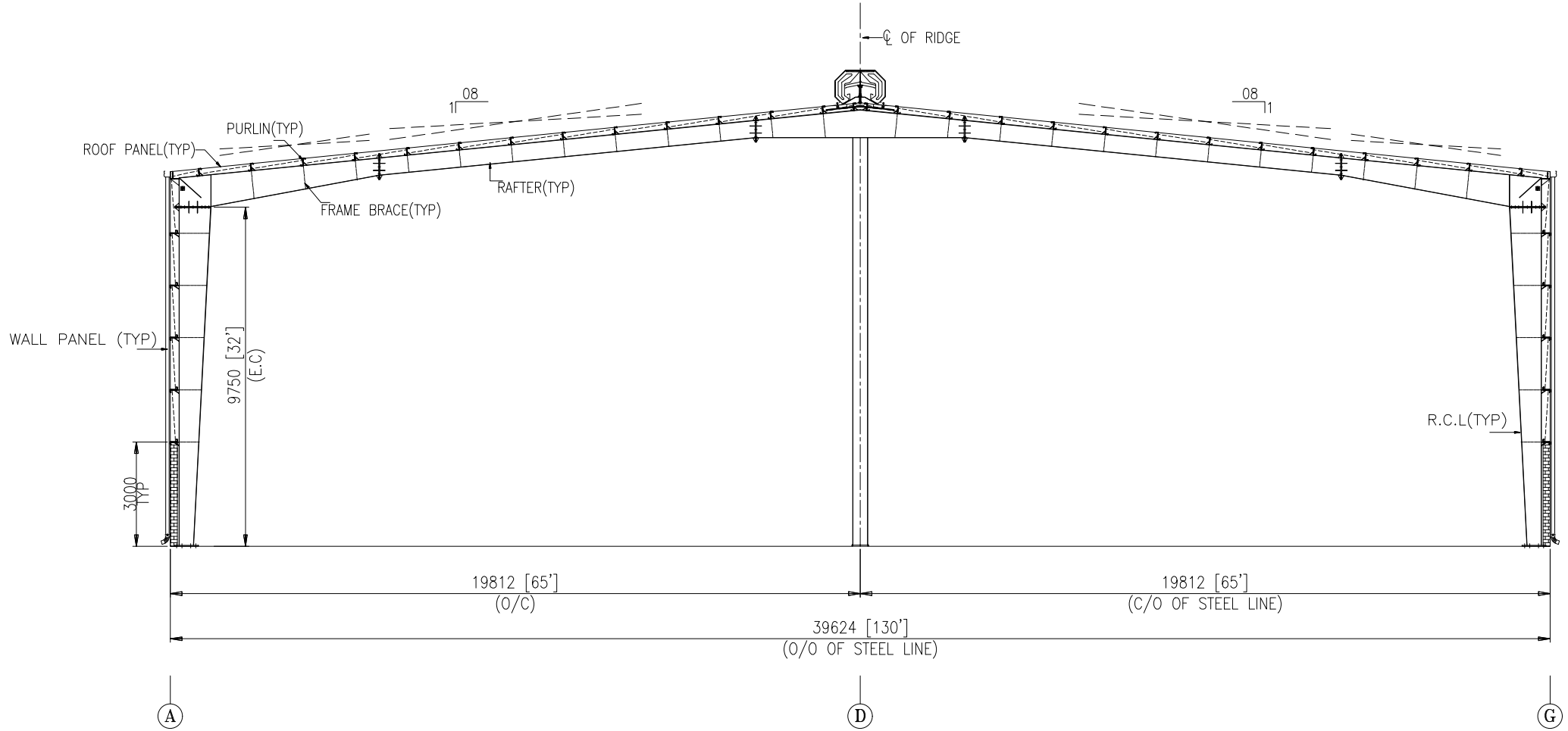
CROSS SECTION AT FRAME LINE-10
